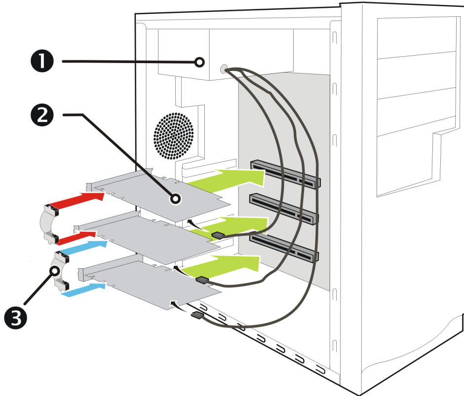
Figure 2-2 ATI CrossFireX Installation
